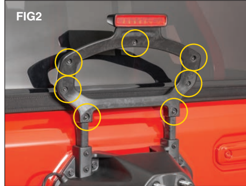
Remove the 7 screws holding the 3rd brake light bracket together using a T-25 Torx driver. (FIG 2)
