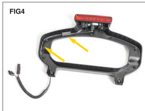
Route and secure the "Y" harness into the channel on the backside of the brake light just as the original harness was. (FIG 4) Connect to the original 3rd brake light.
