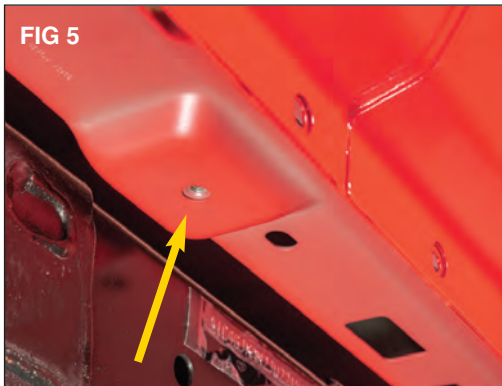
At the rear of vehicle locate the vertical threaded hole behind the pinch weld. (FIG 5)
