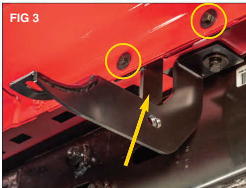
Locate and loosely install the front support bracket (behind) using 6mm hex head bolts (B) through the pinch weld with washers (I) on both sides and secure with a 6mm nylock nut (F) using a 10mm hex wrench and a 10mm socket. (FIG 3)
