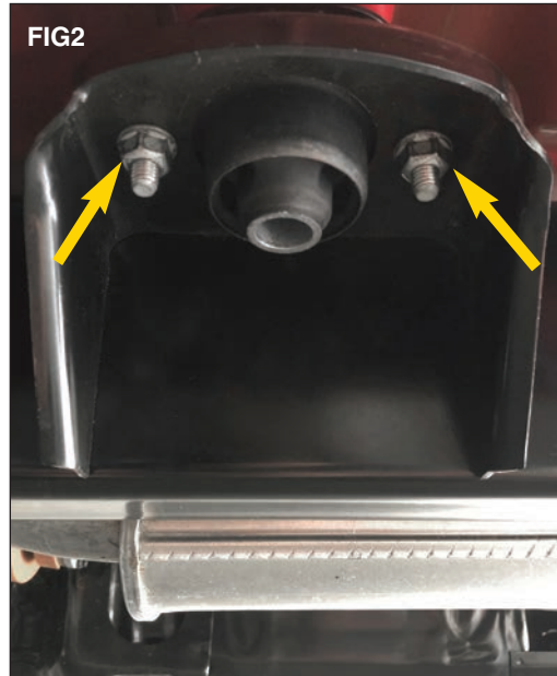
Remove the smaller body mount nuts along the frame using a 16mm socket. (FIG 2) Save hardware.
