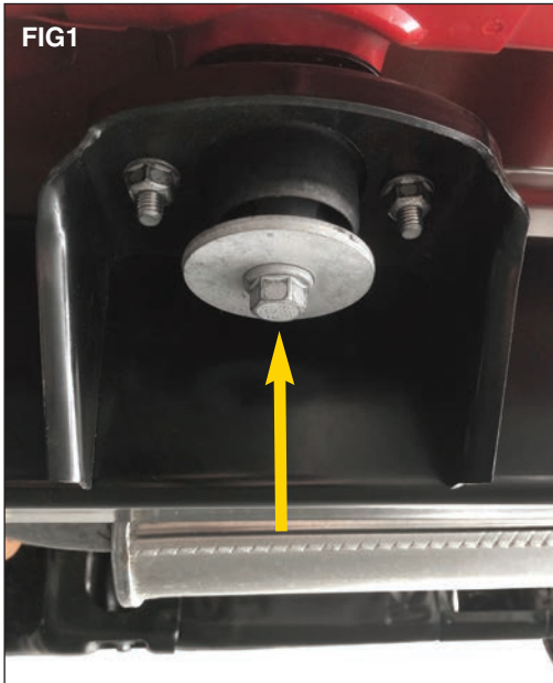
Remove the larger body mount bolts along the frame using a 18mm socket. (FIG 1) You may need to pull down on the large washer as you're backing out the bolt for removal. Save hardware.
