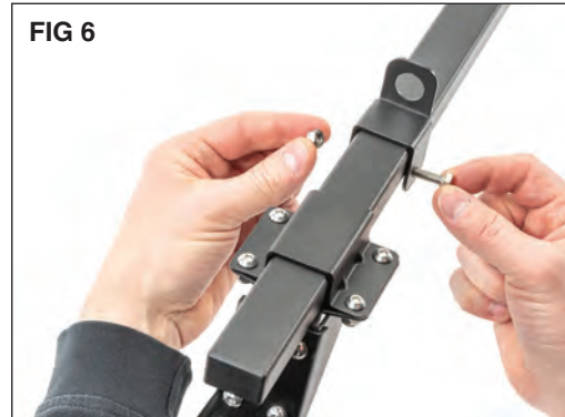
Attach the optional tie down loop to the crossbar with a hex bolt and nylock nut. (FIG6)
